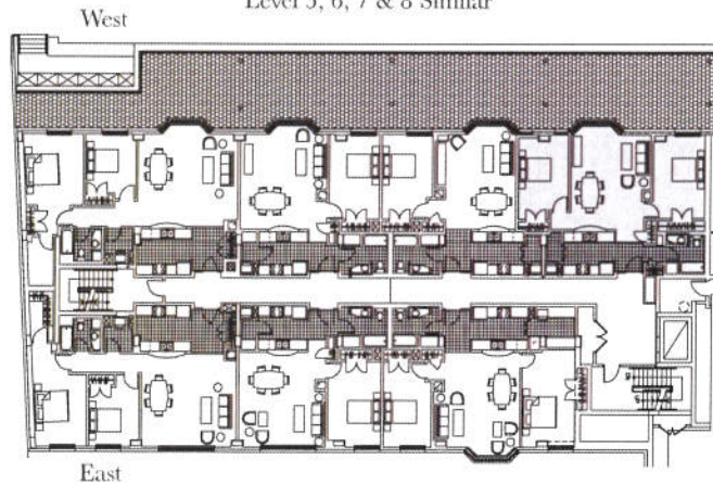
LEVEL 4 Level 5, 6, 7 & 8 Similar
